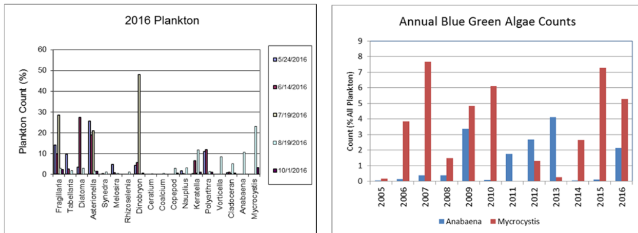
Fig. 9. Date averaged plankton data for 2016 (left) and the mean annual abundance of blue-green algae species since 2005 (right).
