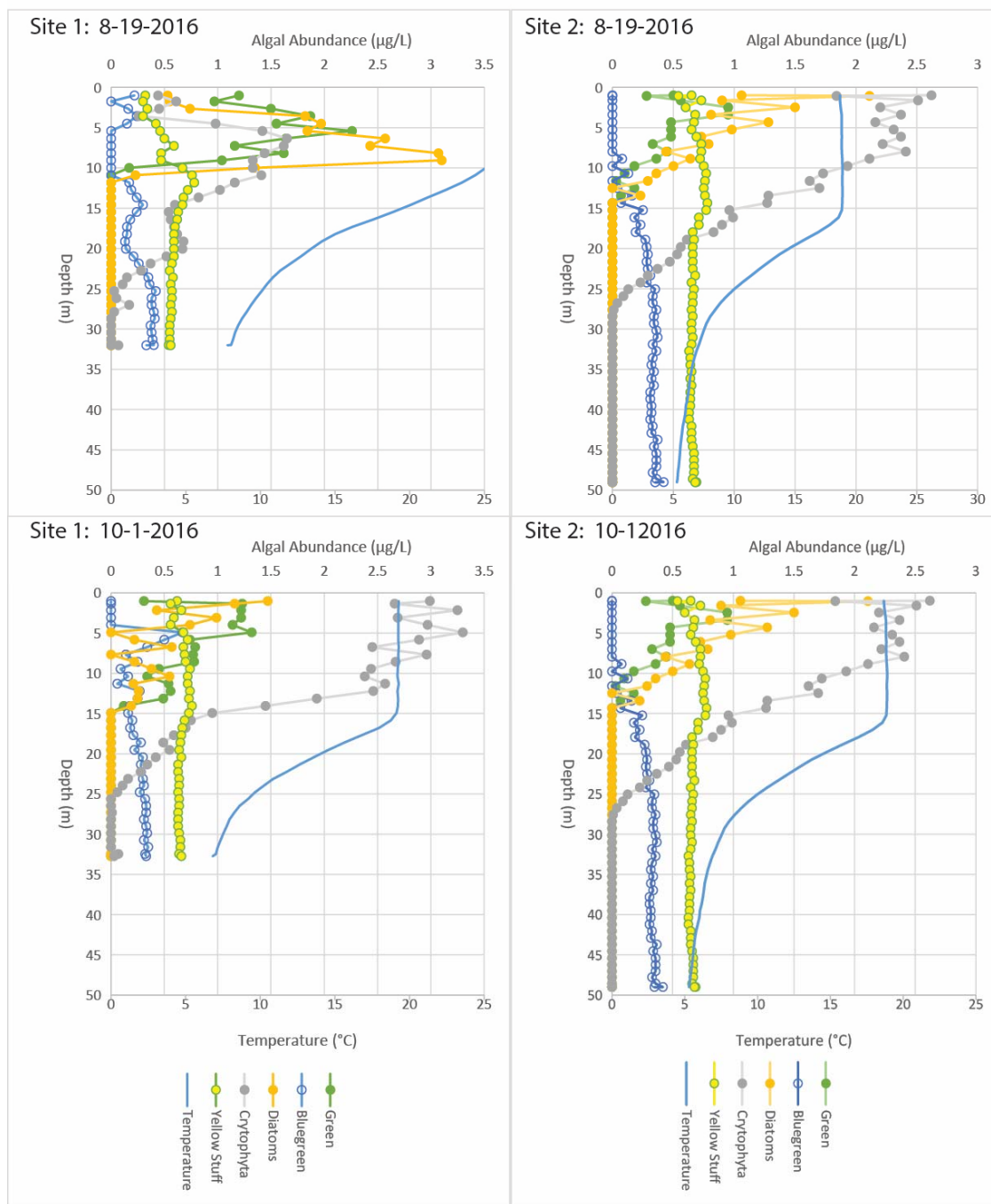
Fig. 6. Fluoroprobe data from Sites 1 & 2 that reveal concentration profiles of four major algal groups.
