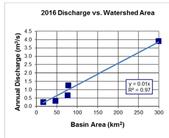
Fig. 18. Discharge vs. Basin Size.
