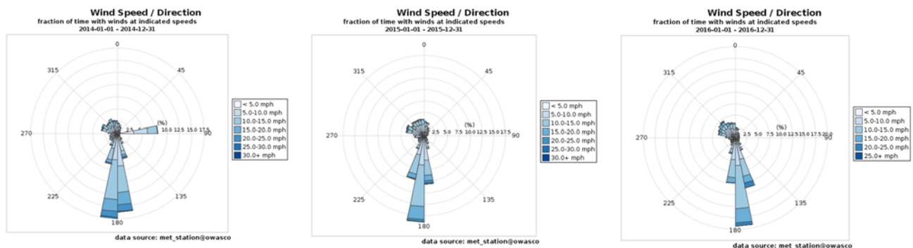
Fig. 16. Wind rose diagrams showing frequency of wind direction and speed for 2014 (left), 2015 (center) and 2016 (right) from the Owasco Lake buoy.
