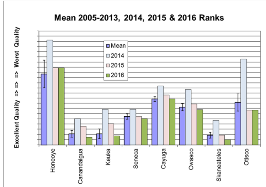
Fig. 10. Annual Water Quality Ranks from 2005 – 2016 for the eight easternmost Finger Lakes. The “mean” dark blue bar averaged the 2005 - 2013 ranks for each lake with a 1\sigma standard deviation error bar.
