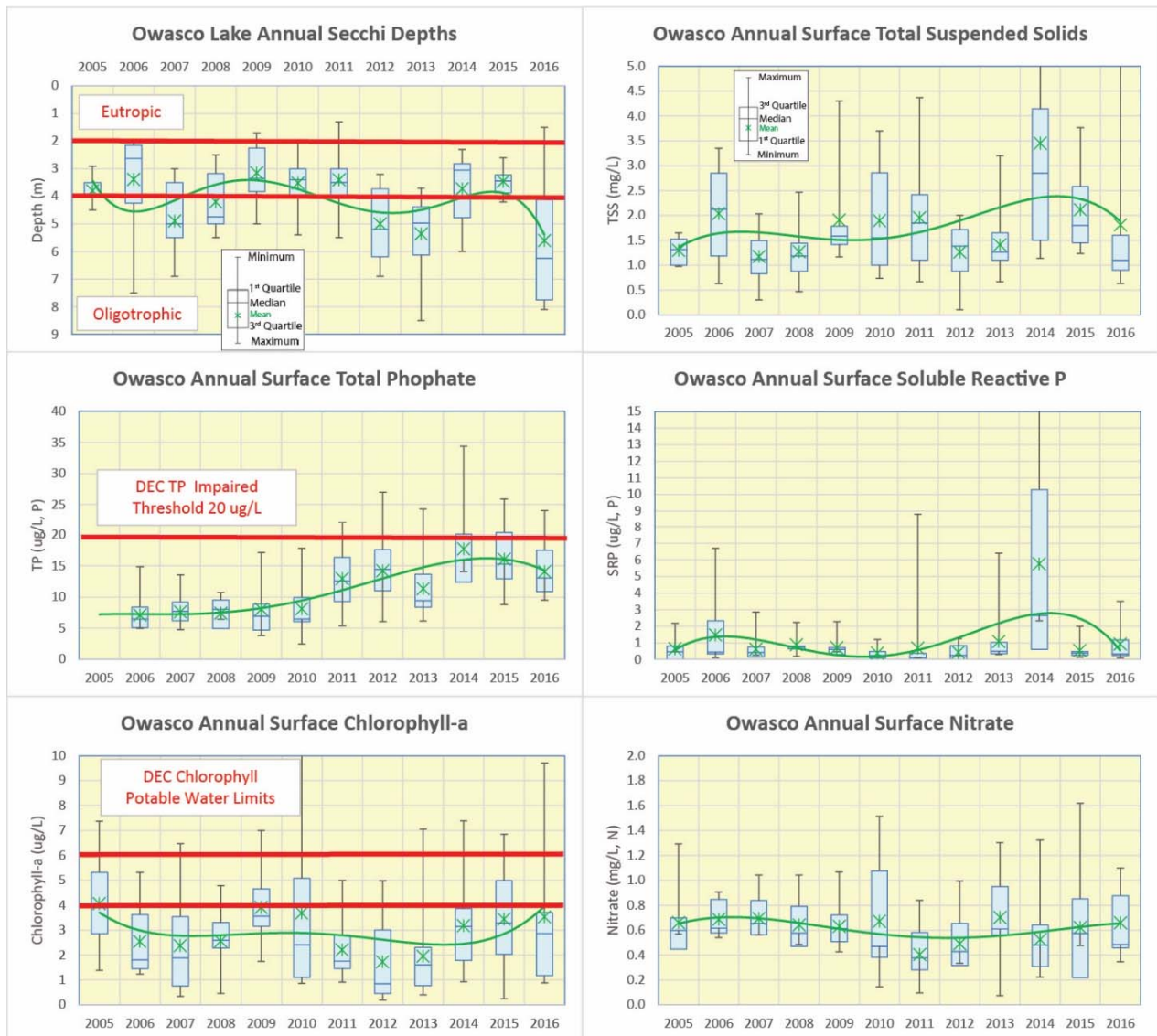
Fig. 8. Box and whisker plots of the lake data.
