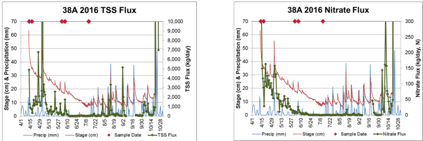
Fig. 31. Autosampler nutrient and suspended sediment fluxes.
