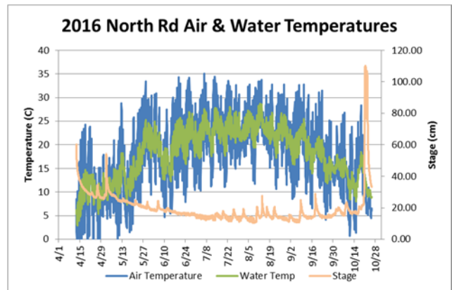
Fig. 28b. Data logger stage and water & air temperature data at North Rd. The seasonal cold to warm to cold cycle prevails.
