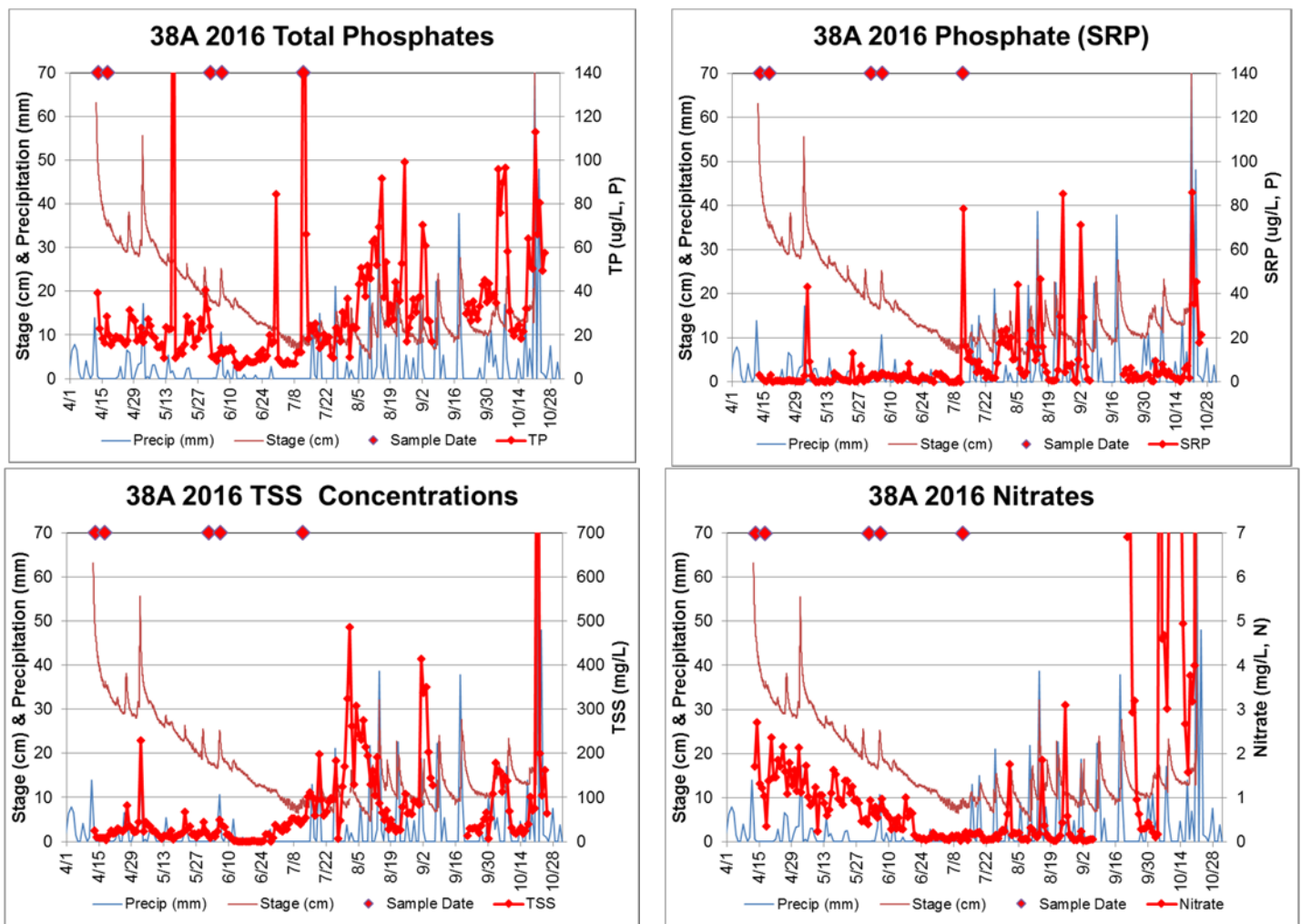
Fig. 29. Rt 38A nutrient and suspended sediment concentrations.
