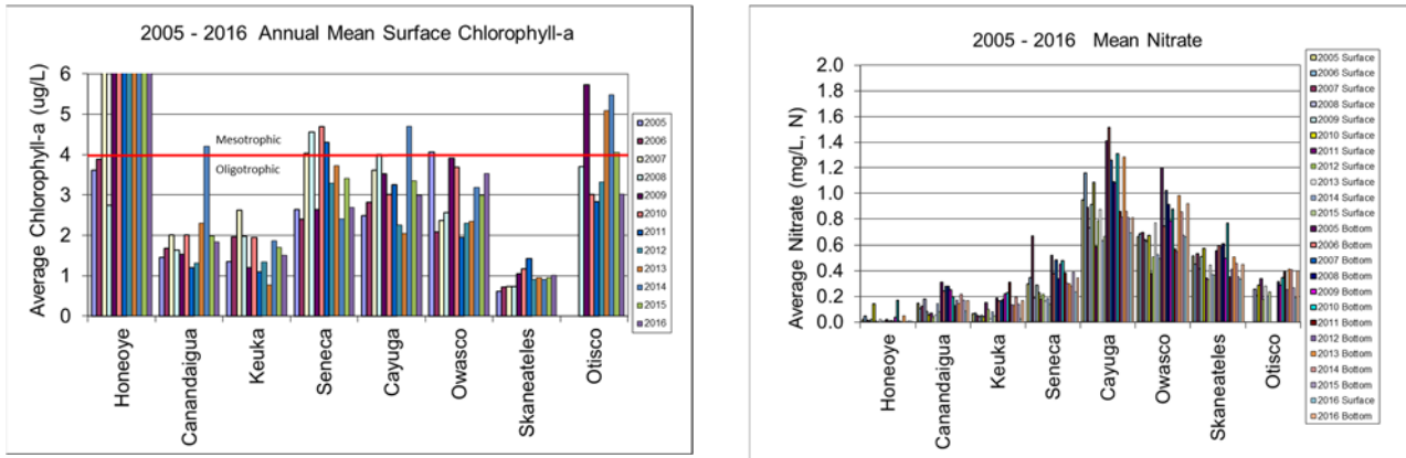
Fig. 11. Annual mean limnological data from selected Finger Lakes. When appropriate, boundaries for oligotrophic, mesotrophic and eutrophic conditions are shown.
