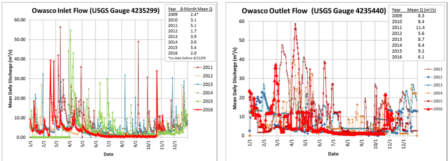
Fig. 23. Annual average stream discharge for the Owasco Inlet near Moravia – USGS Stream Gauge 4235299 and the Owasco Outlet – USGS Stream Gauge 4235440.
