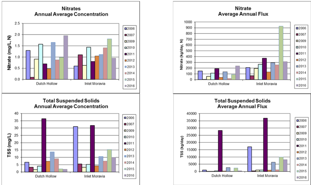
Fig. 26. Annual average stream grab sample concentrations (left) and fluxes (right).
