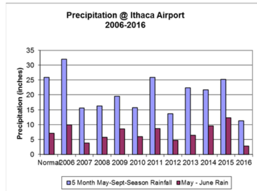
Fig 20. Monthly and “normal” precipitation totals for the Ithaca Airport.
